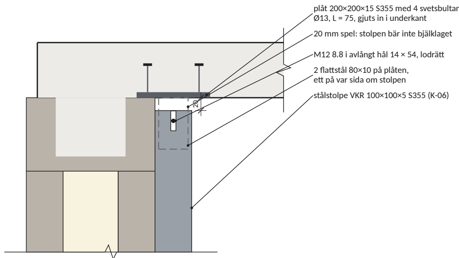
DETALJ E Stålstolpens topp, system A (K-06)
